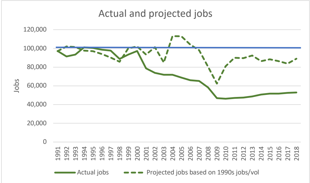
Figure 2. Jobs projected based on annual volume harvested and jobs per cubic metre values (1.3 jobs/thousand cubic metres 1990s baseline) compared to actual jobs. The blue line represents the maximum jobs in the past three decades.
